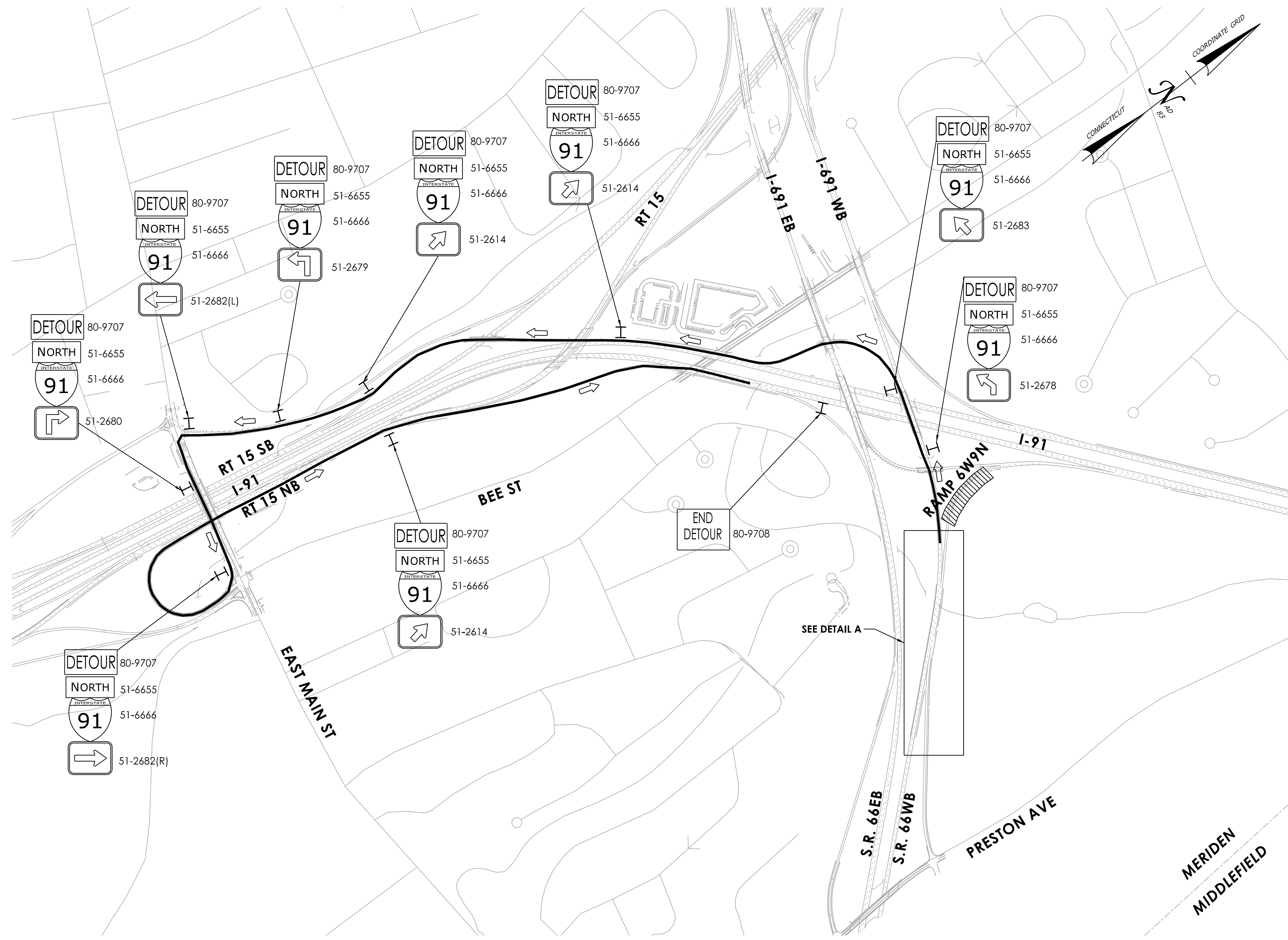
DETOUR PLAN FOR RAMP 6W9N OVERNIGHT CLOSURE NOT TO SCALE
