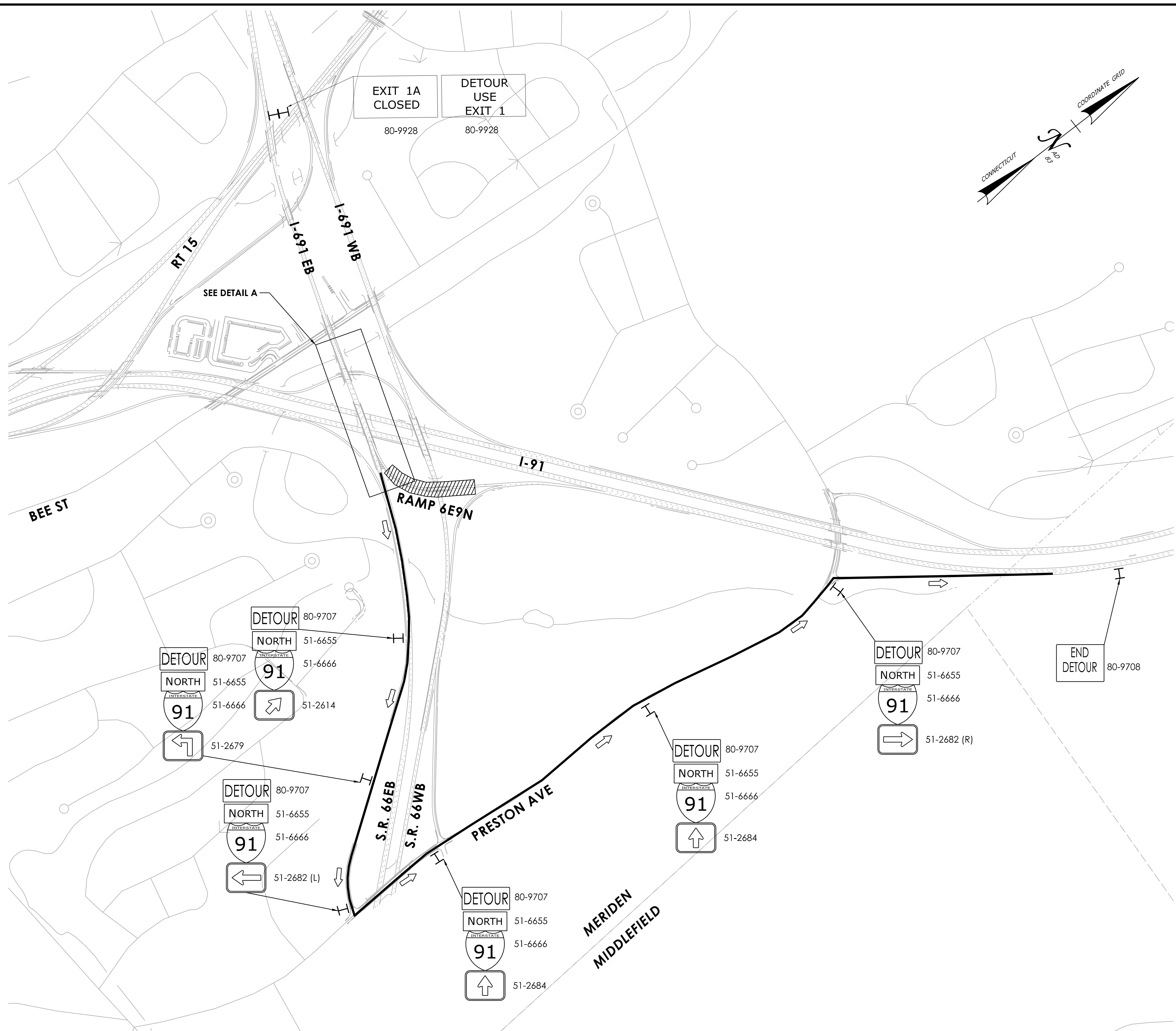
DETOUR PLAN FOR RAMP 6E9N OVERNIGHT CLOSURE NOT TO SCALE
